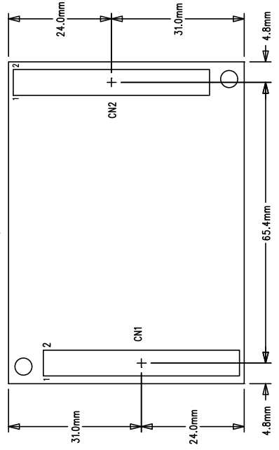
Connector Placement Top View
