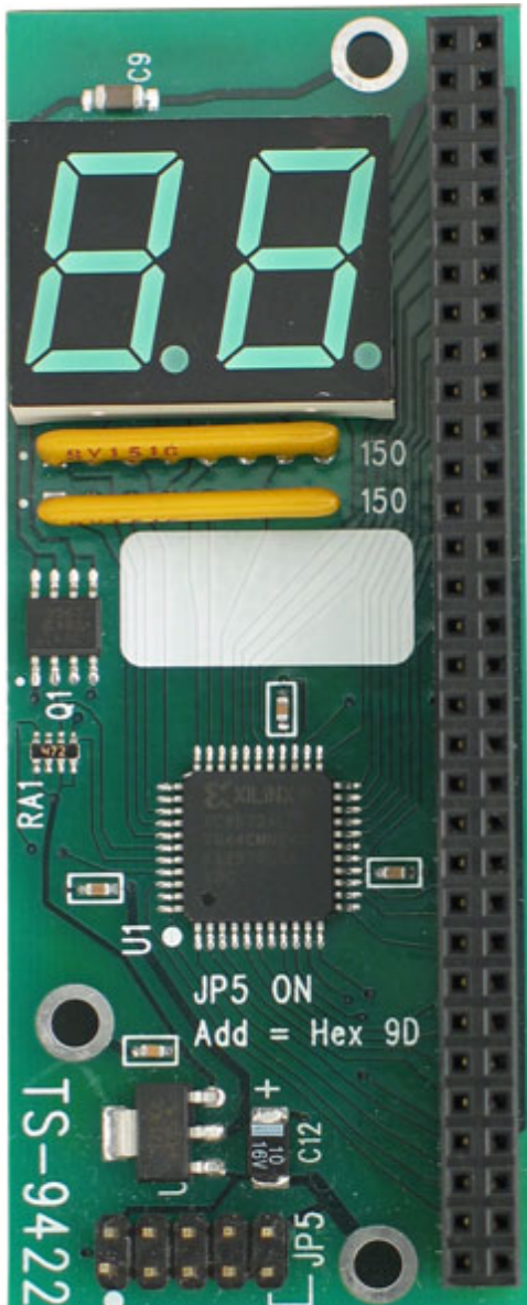
TS-9442 board's front view
