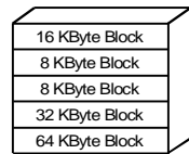
AMD Am29F100T Memory Map No RFD
